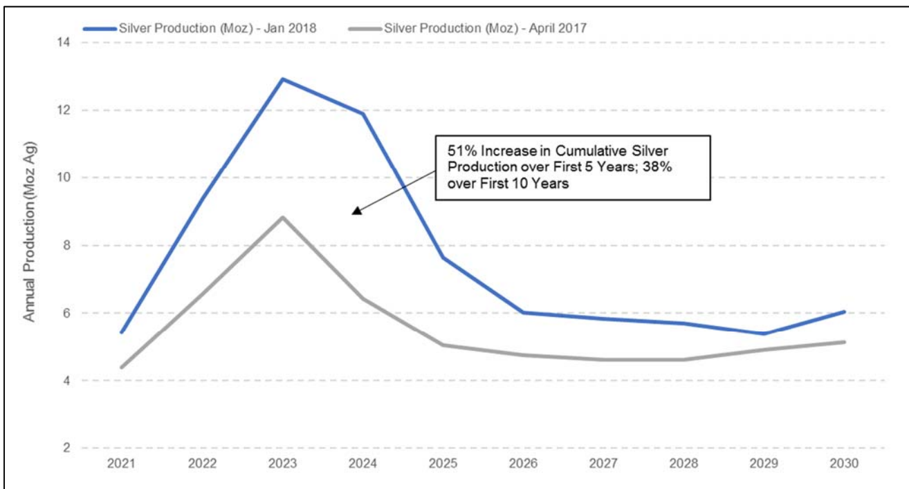
Figure 5. Significantly Enhanced Silver Production in Concentrate – First 10 Years of Mine Life
